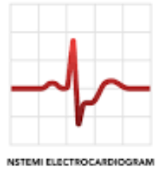
NSTEMI ELECTROCARDIOGRAM
