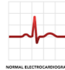
NORMAL ELECTROCARDIOGRAM
